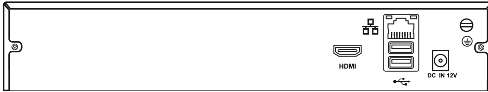
Rear Panel
